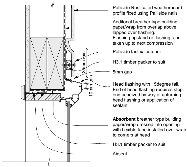
DF01 Window Head Palliside Rusticated profile
