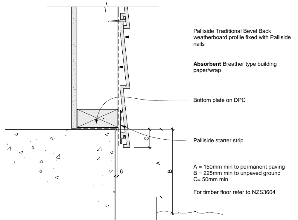
DF05 Ground clearances / Starter strip Palliside Traditional Bevel Back profile
