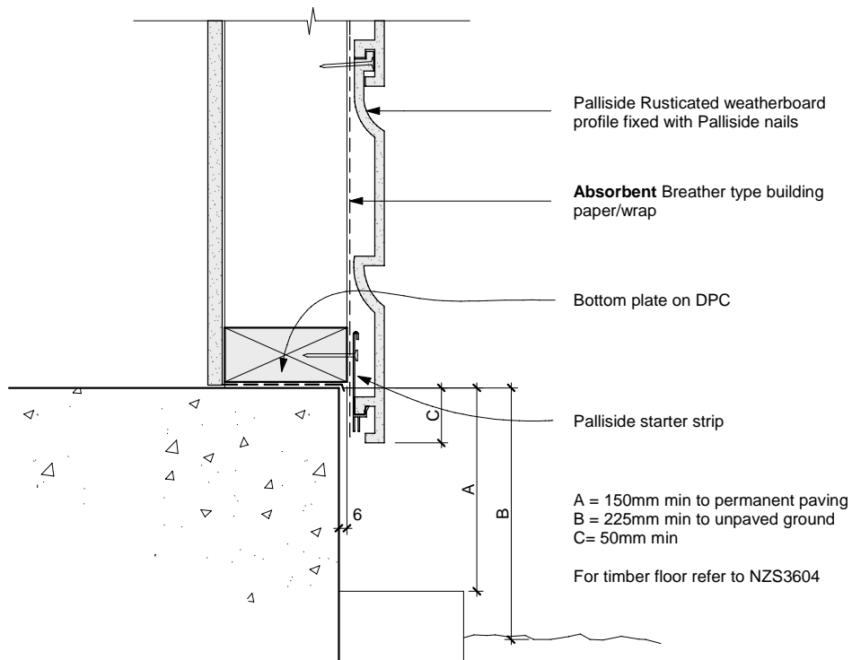
DF05 Ground clearances / Starter strip Palliside Rusticated profile
