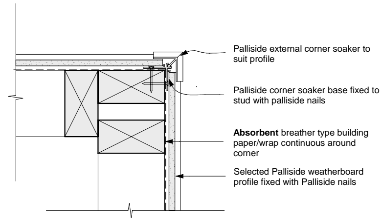
DF06 External corner - Soaker option
