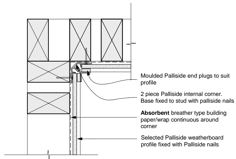
DF08 Internal corner - 2 Part Boxed option
