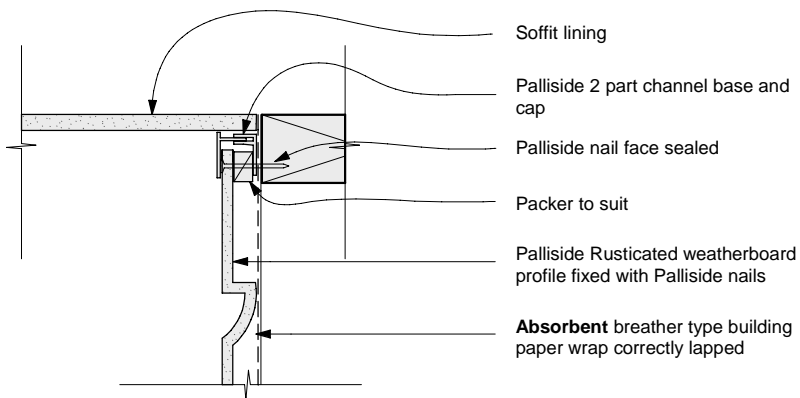
DF11 Finish at Soffit Palliside Rusticated profile
