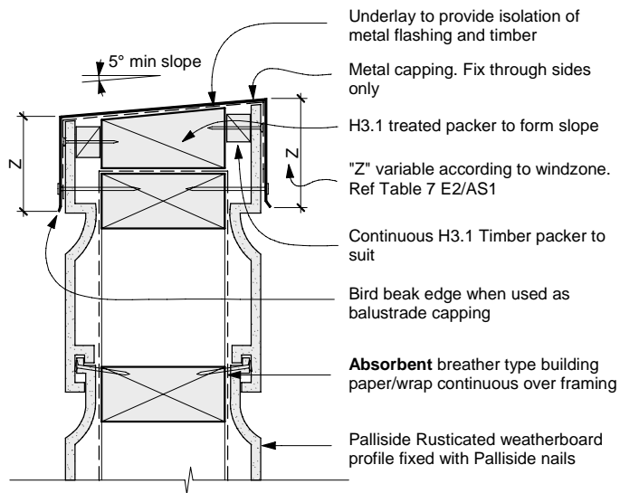
DF12 Parapet and Enclosed Balustrade Palliside Rusted profile
