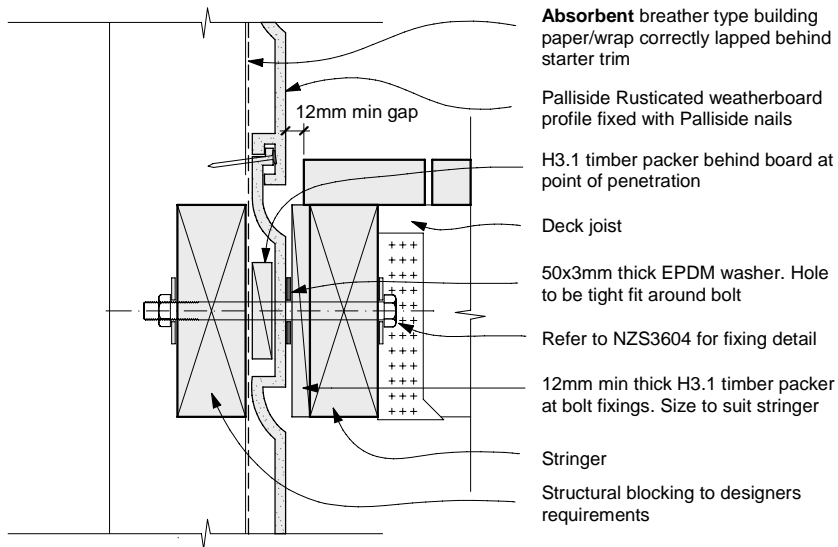
DF16 Wall - Non-cantilevered Timber Deck Palliside Rusticated profile
