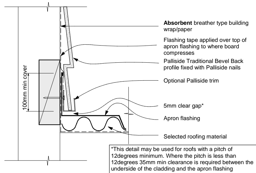
DF17 Apron Flashing - Raked Palliside Traditional Bevel Back profile
