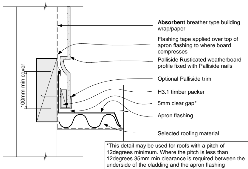
DF17 Apron Flashing - Raked Palliside Rusticated profile
